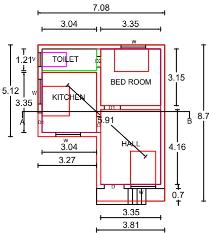
GROND FLOOR PLAN
