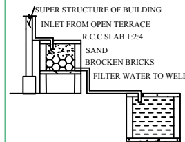
Rainwater harvesting
