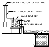
DETAILS OF FILTER BED & WELL
