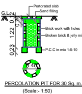
PERCOLATION PIT FOR 30 Sq. m. (Scale:- 1:50)
