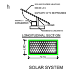
SOLAR SYSTEM
