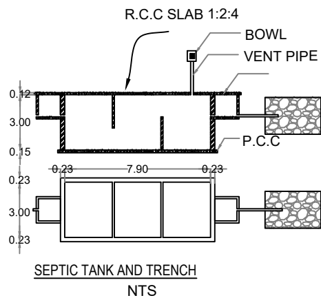
SEPTIC TANK AND TRENCH
