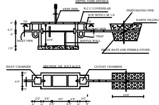
SEPTIC TANK NOT TO SCALE
