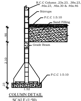
COLUMN DETAIL SCALE:1:50
