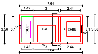
GROND FLOOR PLAN
