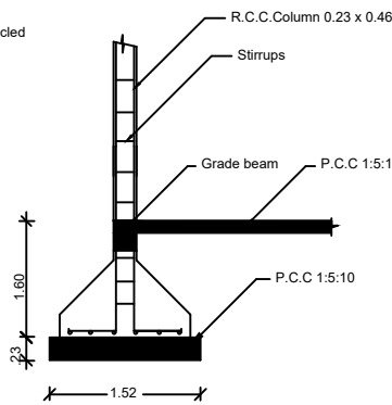
COLUMN DETAIL
