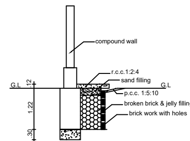
PLINTH BOUNDARY PERCOLATION PIT
