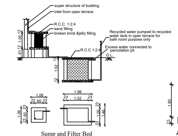
Sump and Filter Bed
