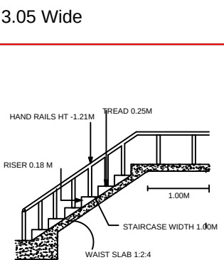
STAIRCASE DETAILS
