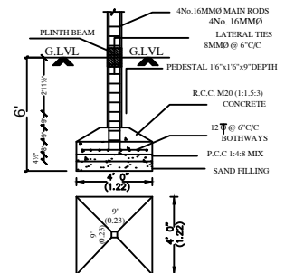
FOUNDATION DETAIL
