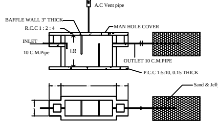
SEPTIC TANK AND TRENCH
