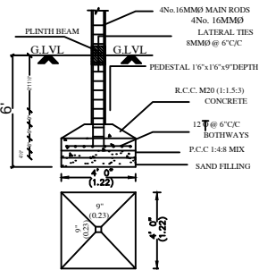
FOUNDATION DETAIL (SCALE: 1:50)
