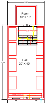
PLAN
