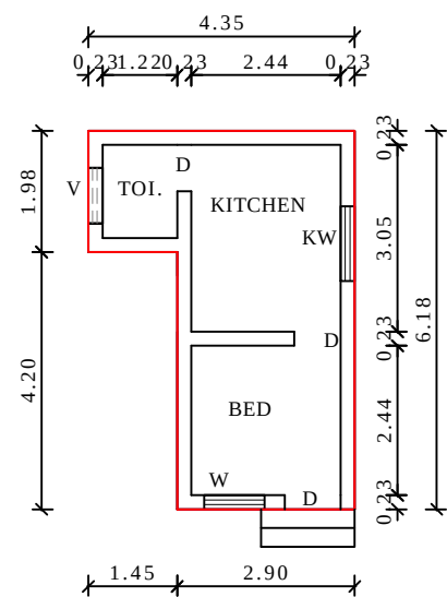
PLAN
