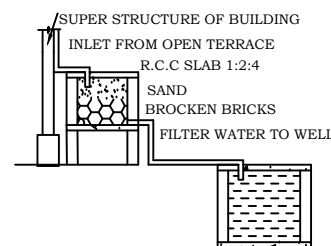
Rainwater harvesting
