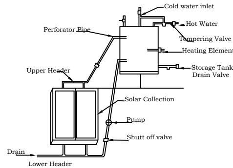
Details Of Solar Water Heater (NTS)
