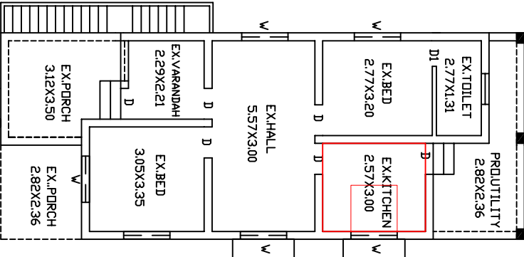
EX.GROUND FLOOR PLAN &PRO.GROUND FLOOR PLAN
