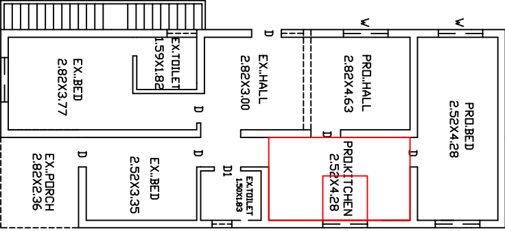
EX.FIRST FLOOR PLAN &PRO.FIRST FLOOR PLAN
