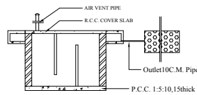
SECTION OF RAIN WATER COLLECTING TANK PLAN
