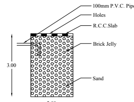
SECTION OF RAIN WATER COLLECTING TANK PLAN
