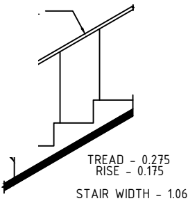
STAIRCASE DETAILS NTS
