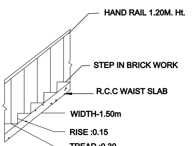
STAIR DETAIL
