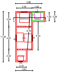
GROND FLOOR PLAN
