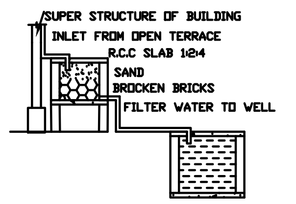
RAINWATER HARVESTING
