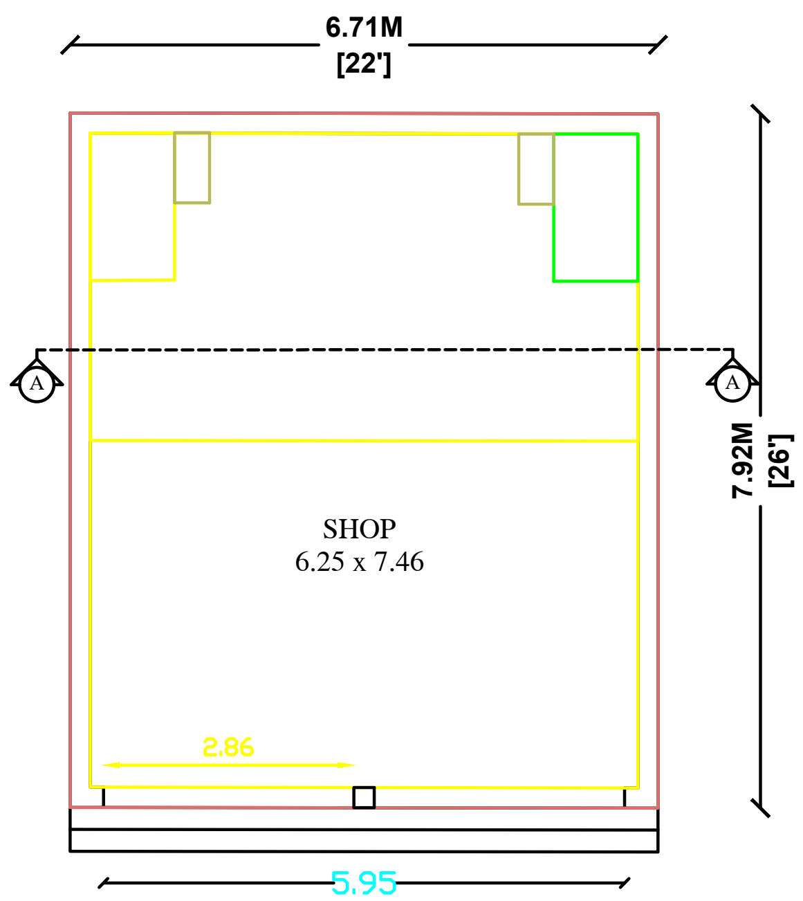
PRO.GOUND FLOOR PLAN
