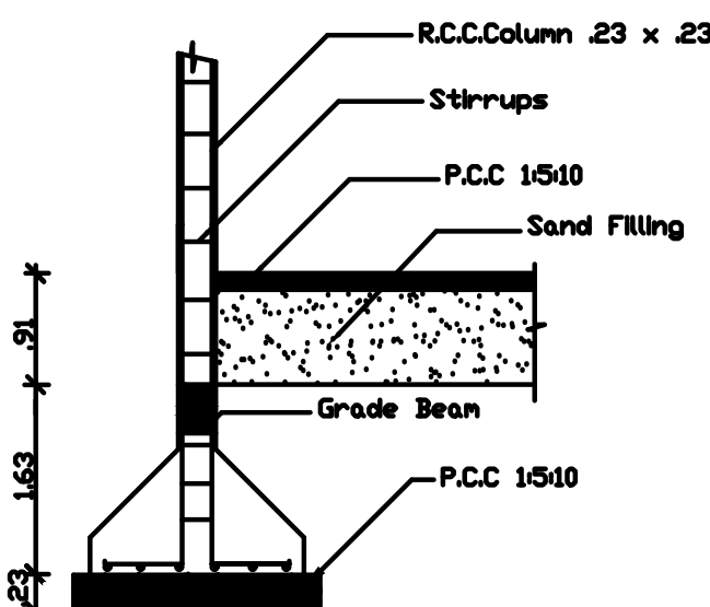
COLUMN DETAIL
