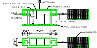
Septic tank and trench
