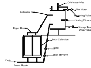
Details Of Solar Water Heater (NTS)
