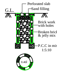
PERCOLATION PIT (NOT FOR SCALE)
