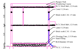
SECTION ON AB
