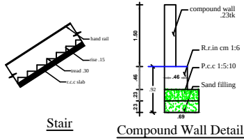
Compound Wall Detail
