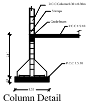
Column Detail
