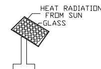
SOLAR SYSTEM
