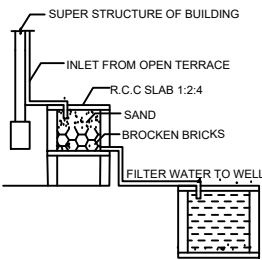
DETAILS OF FILTER BED & WELL NTS
