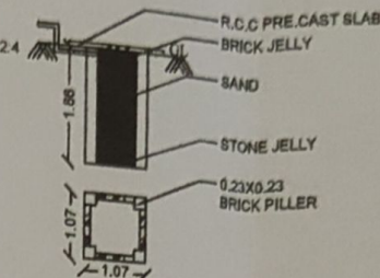
PLAN AND SECTION OF RAINWATER COLLECTION WELL
