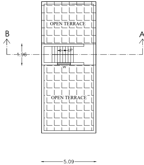
PRO HEAD ROOM PLAN
