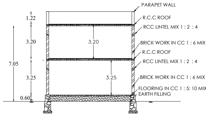
SECTION ON AB & ( HALF ELEVATION)
