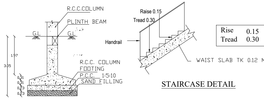
FOUNDATION DETAIL
