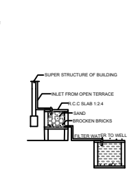
DETAILS OF FILTER BED & WELL
