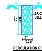
PERCOLATION PIT
