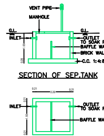
PLAN SEPTIC. TANK
