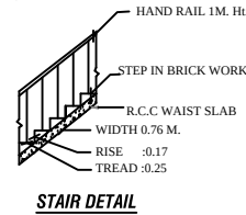
STAIR DETAIL
