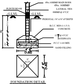
FOUNDATION DETAIL
