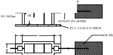
SEPTIC TANK AND TRENCH
