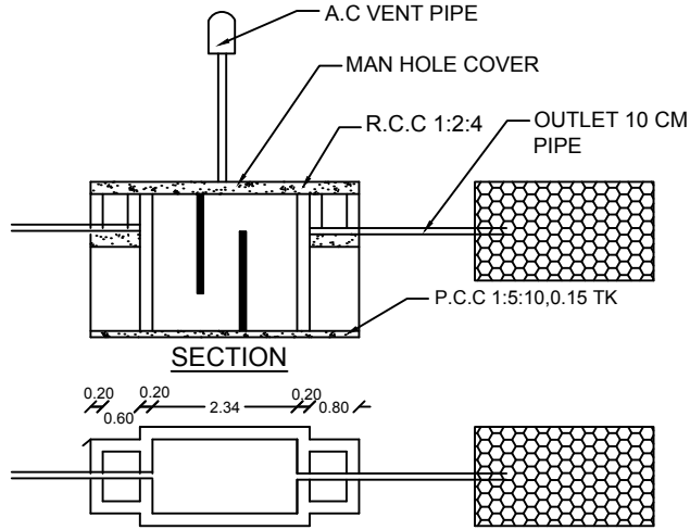
PLAN OF SEPTIC TANK & TRENCH
