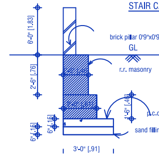
STAIR CASE DETAIL
