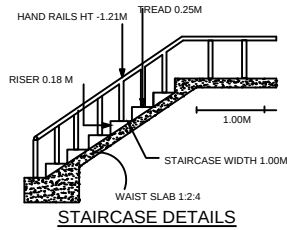
STAIRCASE DETAILS
