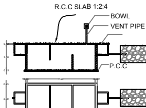
SEPTIC TANK AND TRENCH NTS
