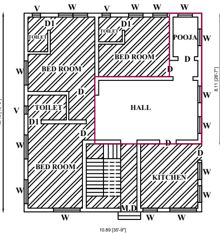
EXG FIRST FLOOR PLAN
