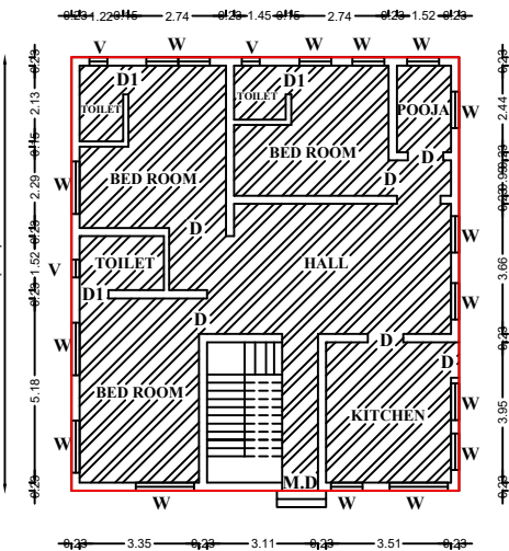
EXG GROUND FLOOR PLAN
