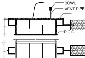
SEPTIC TANK AND TRENCH NTS
