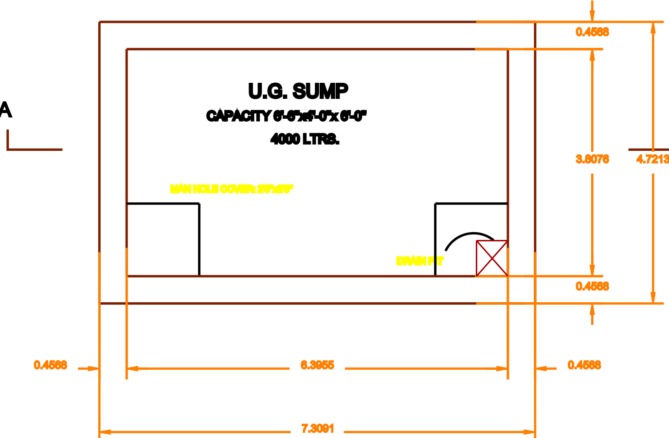
SUMP DETAIL
