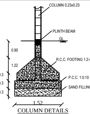
COLUMN DETAILS
