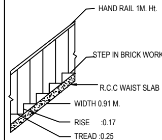
STAIR DETAIL
