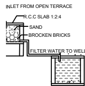
OF FILTER BED & WELL NTS
