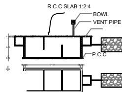
TOILET TANK AND TRENCH NTS
