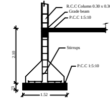
Column Detail
