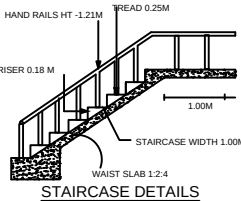
STAIRCASE DETAILS
