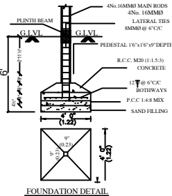
FOUNDATION DETAIL
