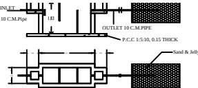
SEPTIC TANK AND TRENCH
