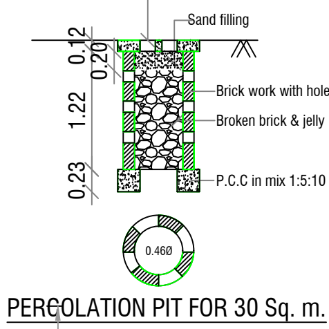
PERCOLATION PIT FOR 30 Sq. m.
