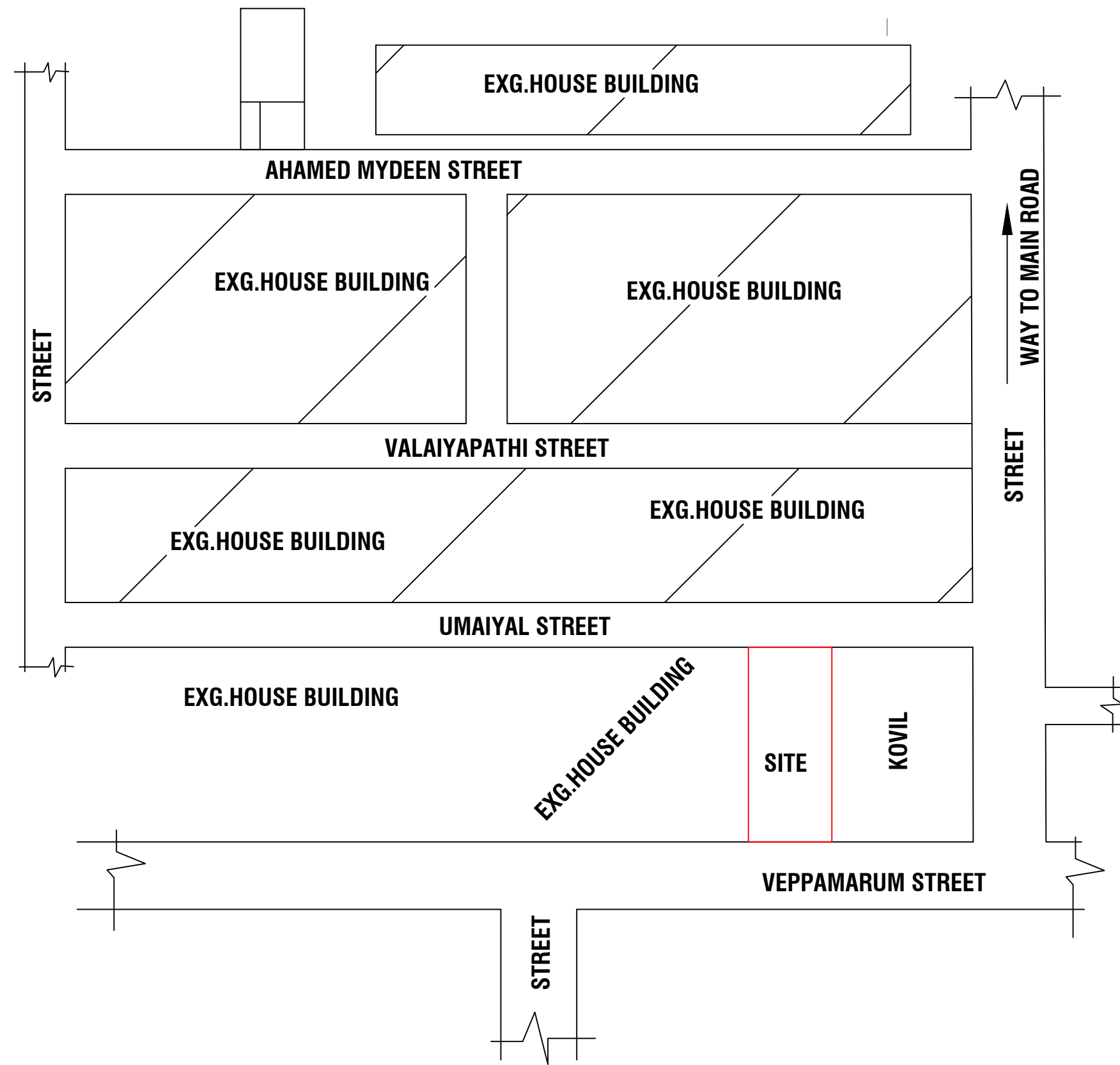
TOPO PLAN/KEY PLAN(NOT TO SCALE)
