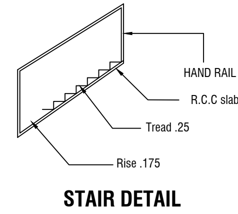
STAIR DETAIL
