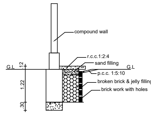
PLINTH BOUNDARY PERCOLATION PIT
