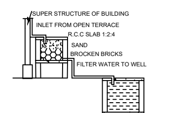
RAINWATER HARVESTING
