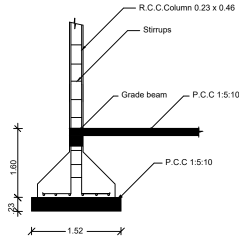
COLUMN DETAIL
