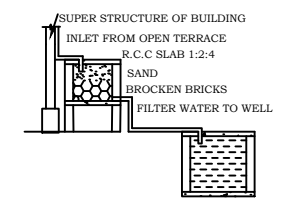
RAINWATER HARVESTING
