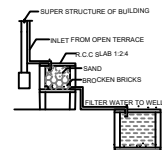
DETAILS OF FILTER BED & WELL N.T.S
