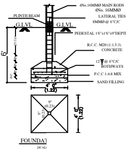
FOUNDATION
