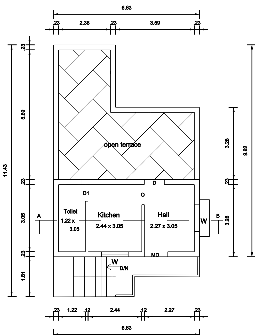
PRO FIRST FLOOR AREA
