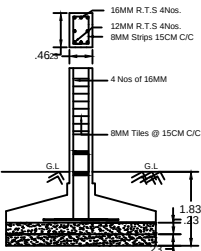
RCC COLUMN DETAILS
