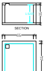
DETAILS OF COLLECTION SUMP FOR RAIN WATER HARVESTING OF ROOF TOP RAIN WATER R.W.H. CAPACITY L=5000LTRS
