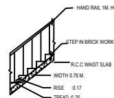
STAIR DETAIL
