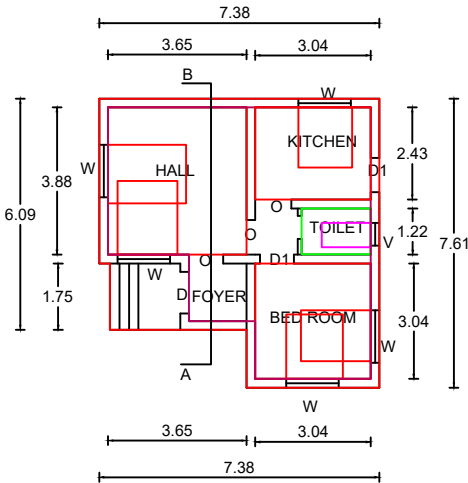
GROND FLOOR PLAN
