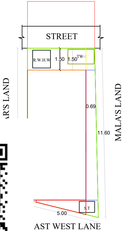
SITE PLAN
