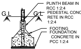
COLUMN DETAILS
