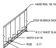
STAIR DETAIL
